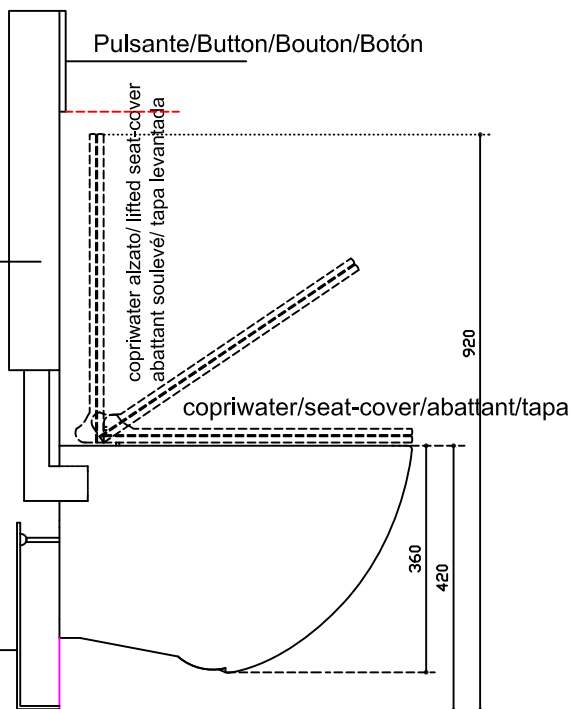
Vista laterale/side view/ Vue lat rale/ Vista lateral
